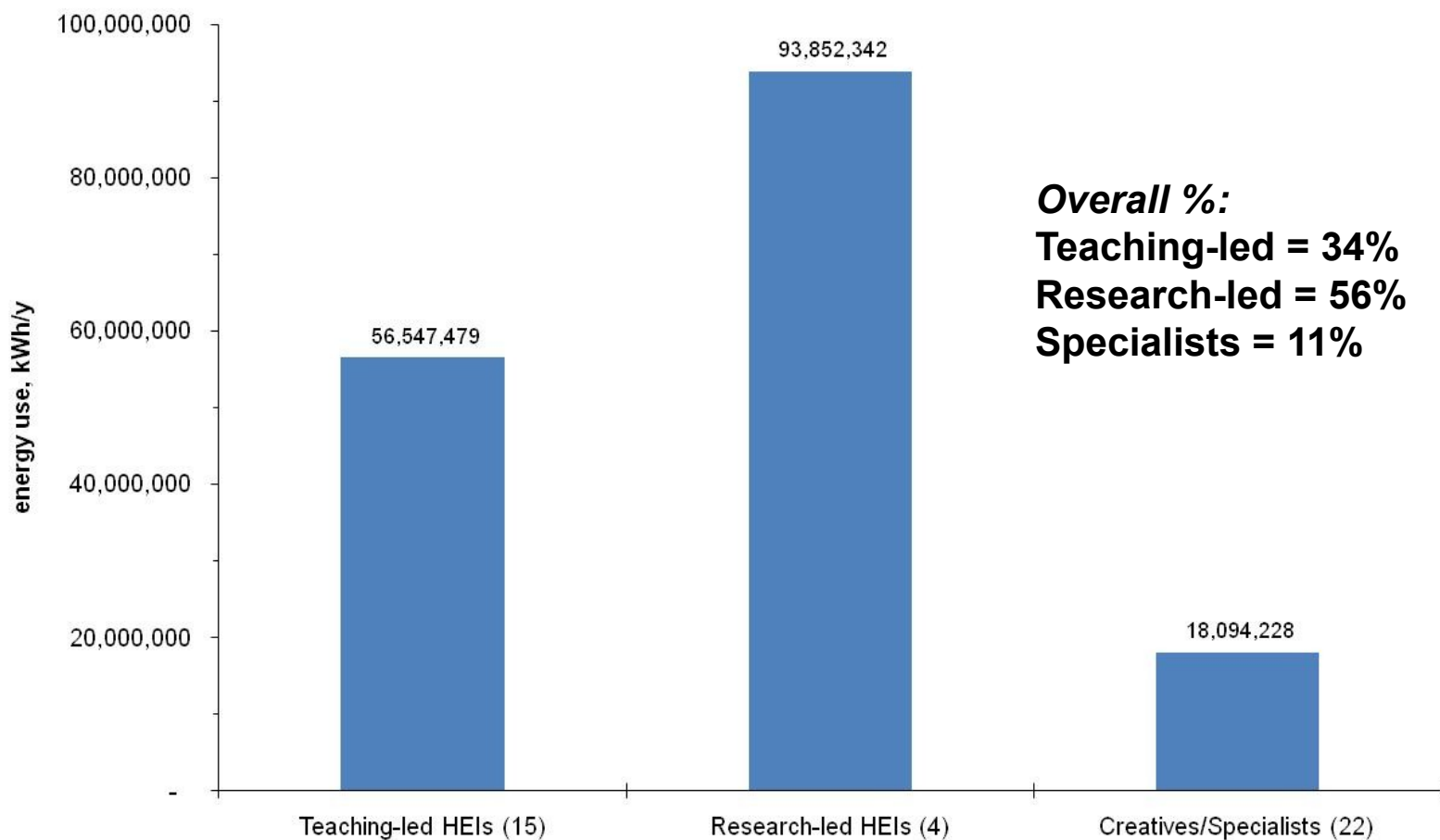
London HEIs: estimated energy use Total = 168,500,000 kWh per year
