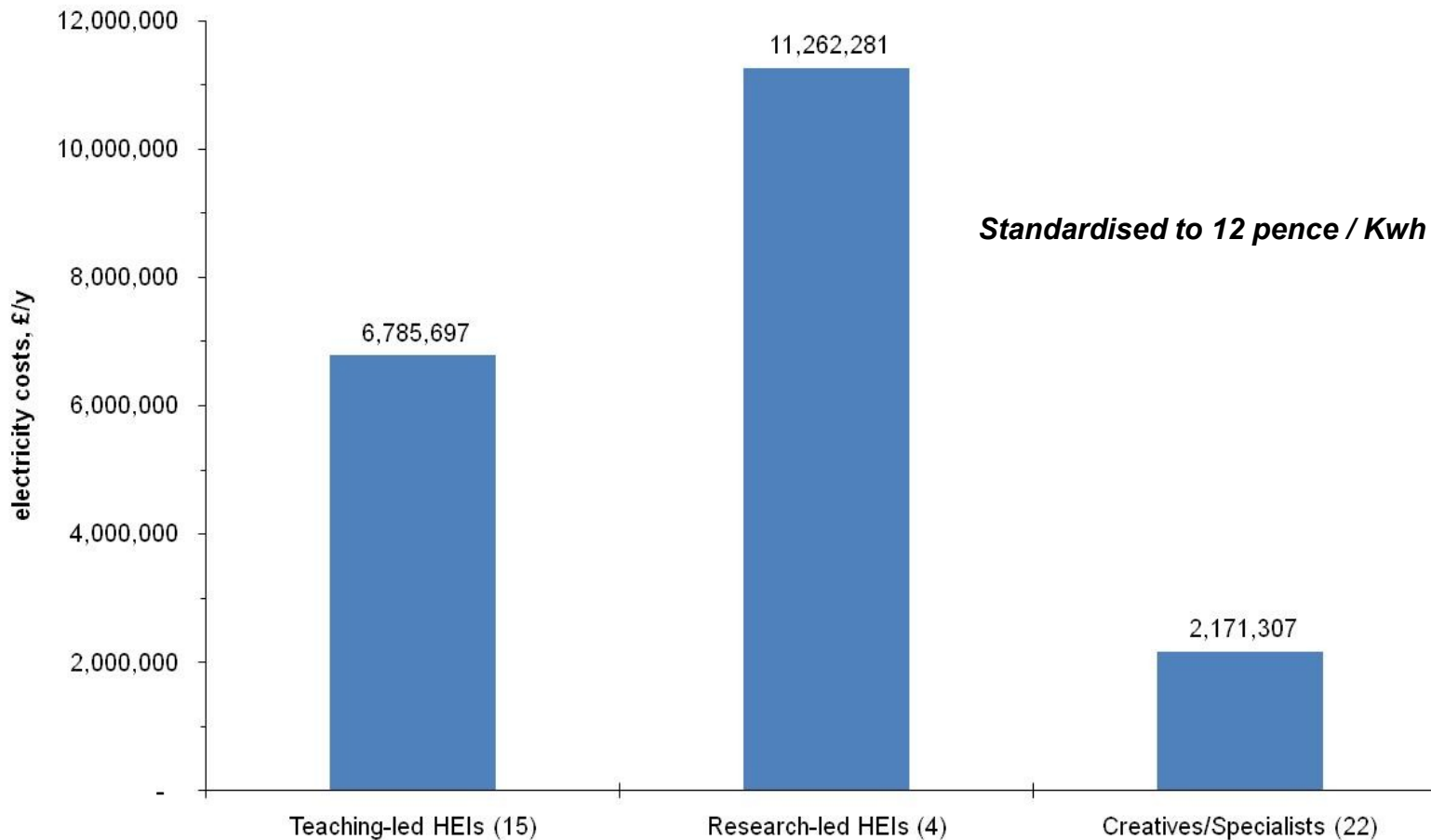
London HEIs: estimated electricity bill Total = £20 million per year
