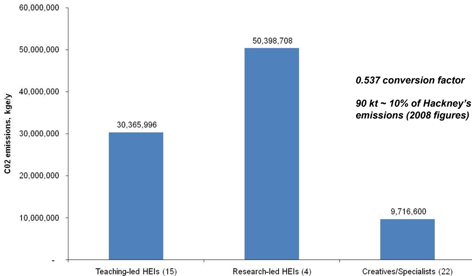
London HEIs: estimated CO 2 emissions Total = 90 million kg per year
